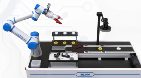
Collaborative Robot Vision Inspection Line
